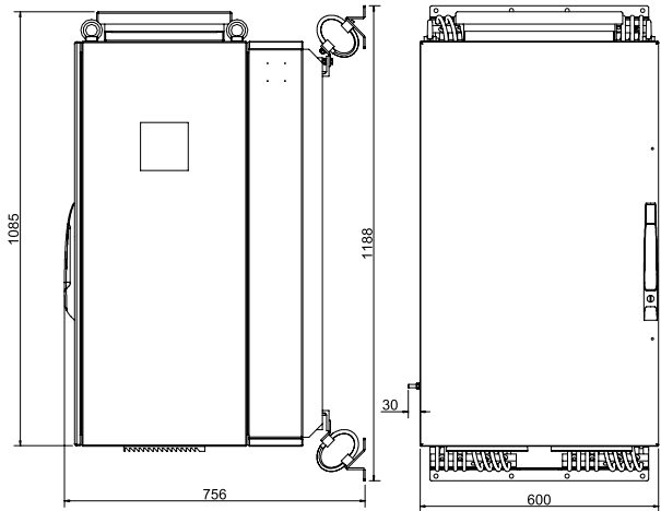
Outline dimensions for Transceiver Unit
