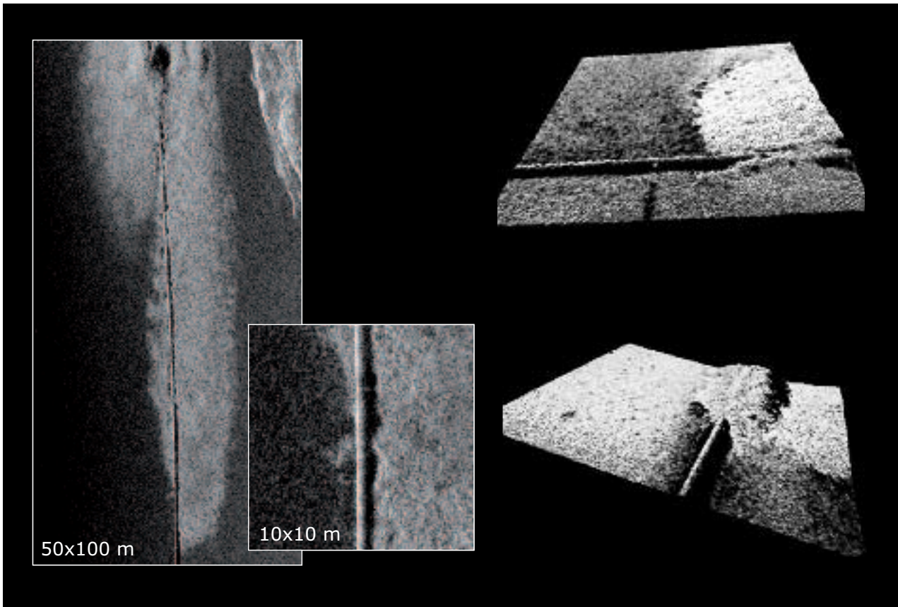
Example of SAS images from pipeline survey operation. 2 nmi x 500 m covered in one hour, with heavy overlap and one pass at each side of the pipeline
