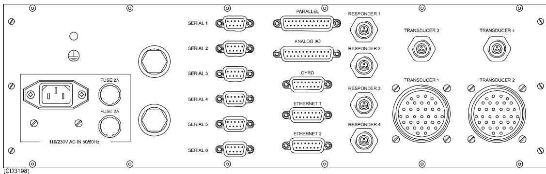
Figure 1 Connectors on the HPR Transceiver Unit's rear panel
