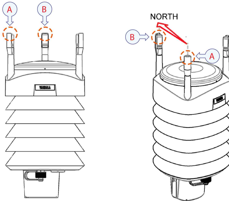
Figure 22 WXT520/530 wind sensor location and rotation direction
