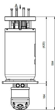
Outline with Nortek DVL 1000 collocated
