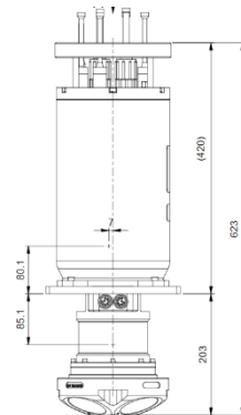
Outline with Nortek DVL 500 collocated
