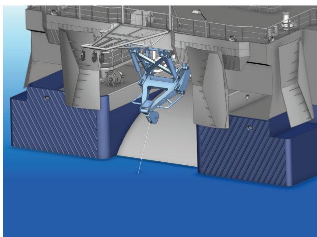
Deployed in low towing position
