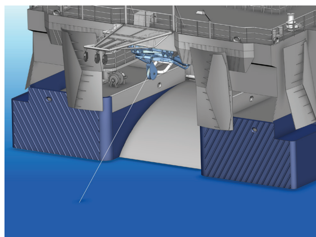
Deployed in high towing position
