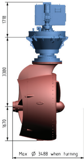
Thruster unit seen from side
